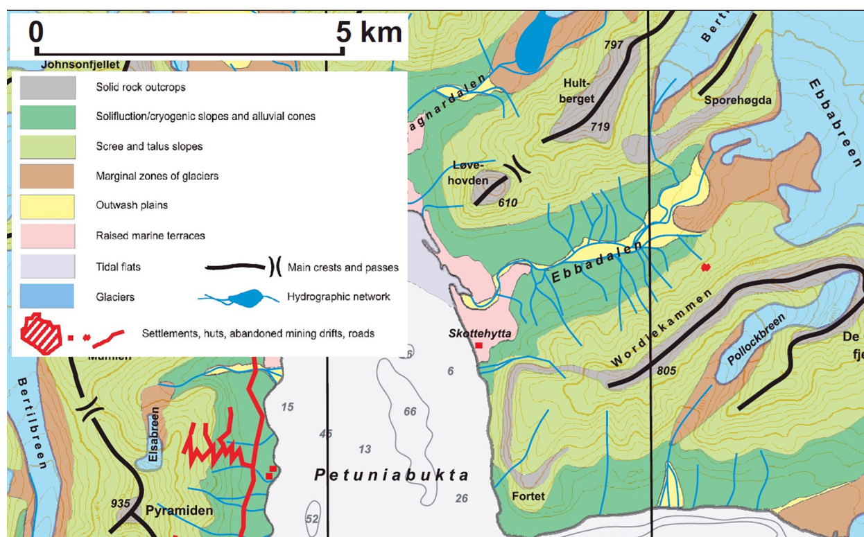
Fig. 2. Geomorphological sketch of the study area (Ebba Valley, Svalbard). Modified after the original figure by Rachlewicz (2009).
